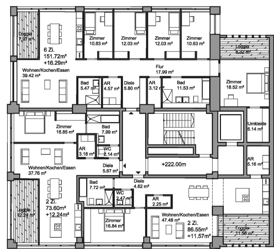
Grundriss RG2 Sudhaus_M 1:200
