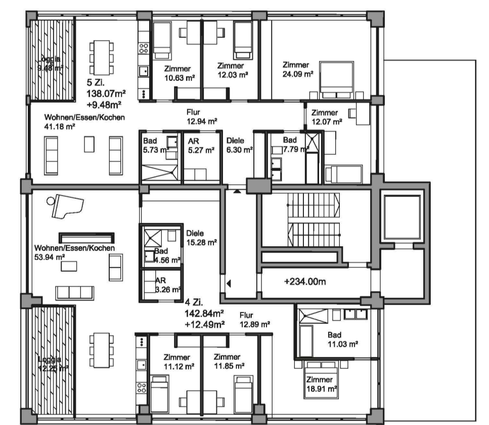
Grundriss RG3 Sudhaus_M 1:200
