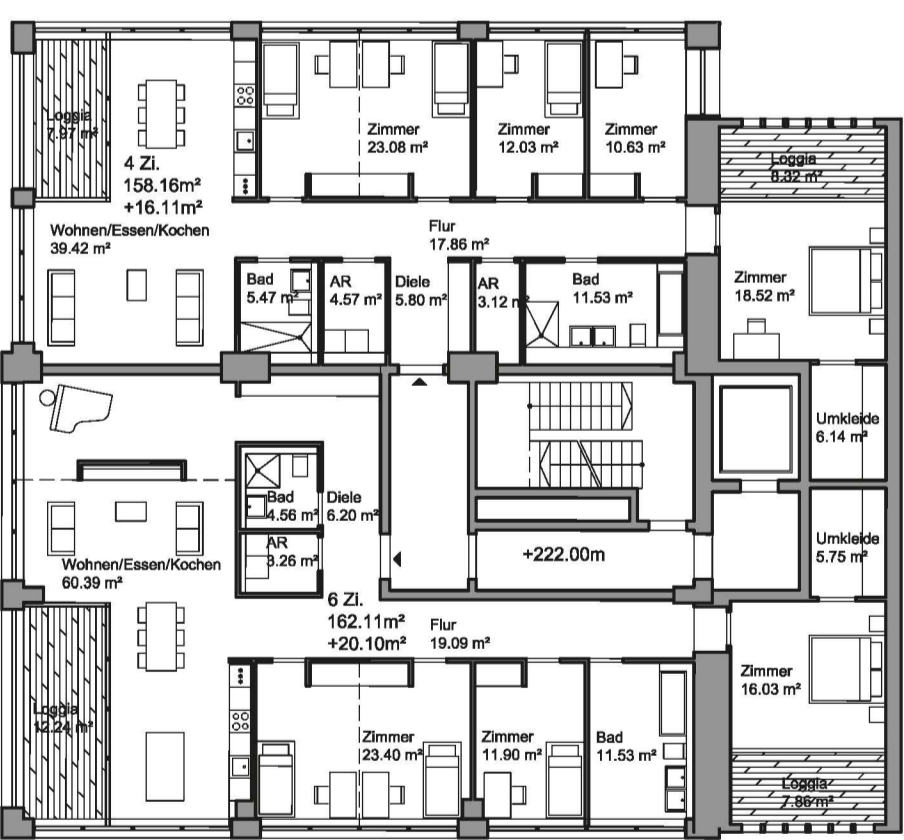
Grundriss RG1 Sudhaus_M 1:200
